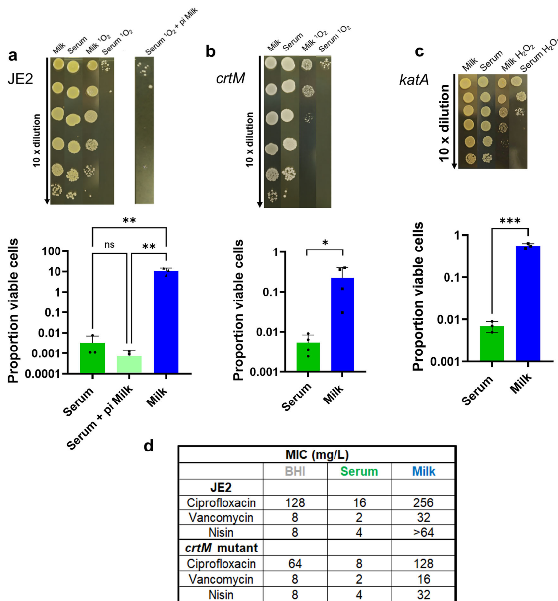
Fig. 6 | Tolerance to ROS and antibiotic is stimulated in milk-grown S. aureus , and diminished in crtM or katA mutants. JE2 WT and mutant cultures prepared in adult bovine serum, or whole milk conditions were washed and resuspended in physiological saline. a WT JE2 and b a crtM transposon mutant 77 bacteria were untreated or exposed to singlet oxygen, and then serially diluted, spotted on BHI agar and grown overnight to determine survival. Note the difference in scale in a and b logarithmic graphs. Experiments were repeated at least three times. For JE2 ( a ) an aliquot of serum-grown bacteria was subject to 1 h exposure to milk and then washed prior to singlet oxygen treatment (at right). Continued high sensitivity allowed us to rule out non-specific effects of milk-bound bacteria. c H 2 O 2 sensitivity was compared in milk- versus serum-grown WT JE2 (Supplementary Fig. 11) and the katA transposon mutant 77 . For a–c results are representative of at least 3 independent
