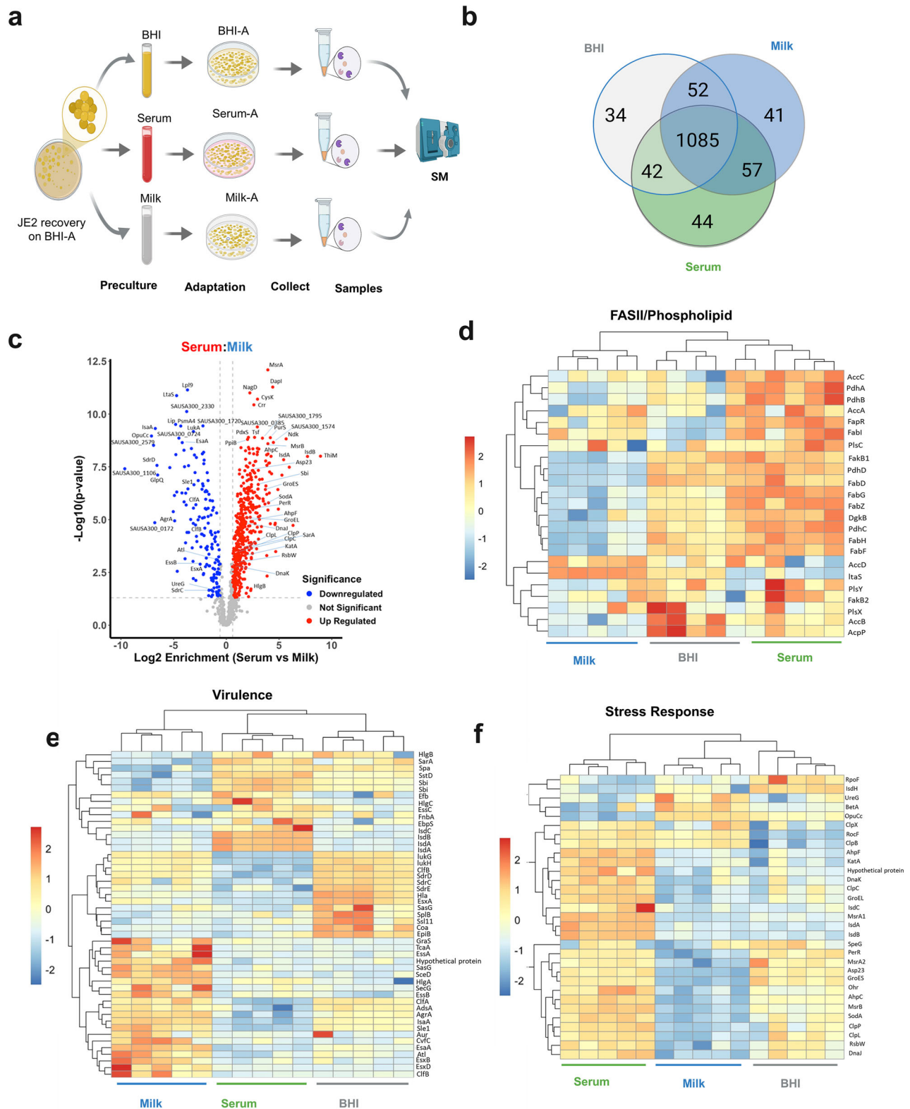
Fig. 4 | Comparative proteomics of BHI-, serum-, and milk-grown S. aureus . a Flowchart for the study. Bacterial grown in the three conditions (BHI, adult bovine serum, or whole milk) and in five independent replicates were harvested from agar plates after overnight cultures and processed for proteomics analysis. Created in BioRender. Vidic, J. (2026) https://BioRender.com/xnjr53d b Venn diagram showing the number of identified proteins detected in each condition, based on the five biological replicates. Full data is presented in Supplementary Data 1. c Volcano plot depicts the magnitude ( \log_2 fold change) and statistical significance ( q -value) comparing levels of the expressed proteins in JE2 between serum- and milk-grown cultures. Horizontal dashed lines
