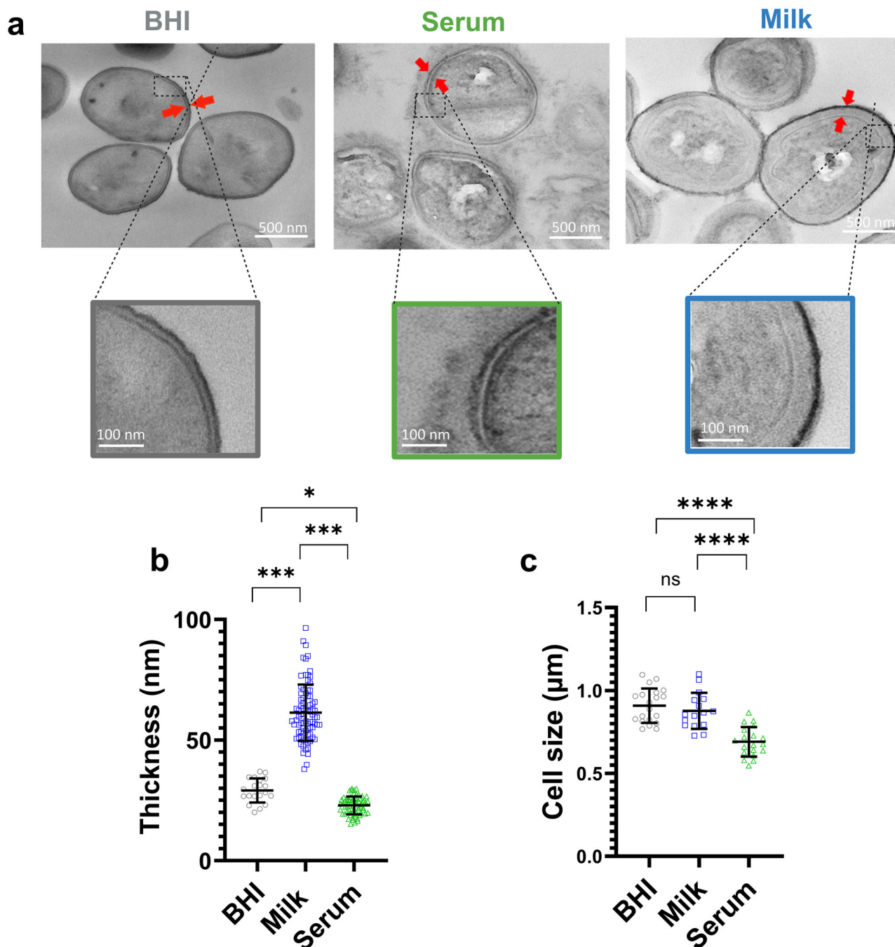
Fig. 2 | Serum and milk modulate S. aureus envelope. a Representative transmission electron microscopy images of milk-grown and serum-grown saturated JE2 bacteria. BHI-grown cells are presented for comparison. Arrows indicate envelope thickness. Scale bar for the upper panels, 500 nm. The zoom illustrates the highly different S. aureus envelope morphology between the 3 conditions. b Range of cell envelope thickness, and c cell sizes of JE2 grown in BHI, adult bovine serum, or
