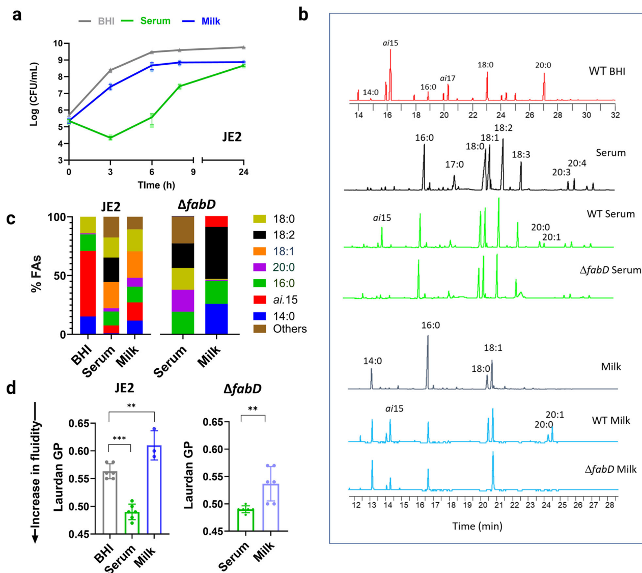
Fig. 1 | S. aureus growth and exogenous FA incorporation in serum or milk. a S. aureus JE2 growth was assessed by determining CFUs in adult bovine serum, whole milk, and BHI liquid medium by plating dilutions on BHI agar at given time points. Data represent mean \pm SD of three independent experiments. b Membrane FA profiles were compared in JE2 (WT) and the \Delta fabD FA auxotrophic derivative grown in serum, milk, or BHI. The JE2 strain cultured in BHI (red profile) synthesizes FAs via FASII, and its FA profile is dominated by ai 15, its elongation products ( ai 17, ai 19) and saturated straight chain FAs (C16:0, C18:0, C20:0). In contrast, JE2 FA profiles in serum (green) or milk (blue), are both enriched with exogenous FAs supplied by the medium. The FA auxotroph \Delta fabD displays a similar FA profile as that of its respective medium. Peak heights correspond to relative
