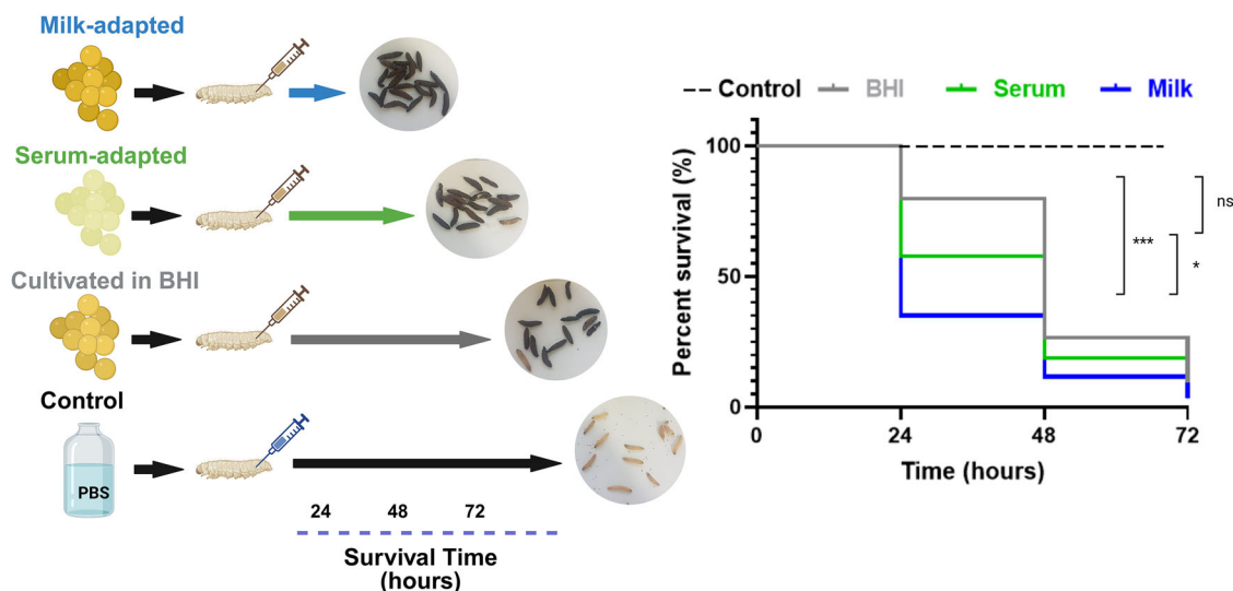
Fig. 7 | The S. aureus environmental origin affects infection efficacy. The infection capacity of adult bovine serum-, or whole milk-, or BHI-grown S. aureus was compared using the G. mellonella infection model. Created in BioRender. Vidic, J. (2026) https://BioRender.com/b5jturg a Schematics of the in vivo infection assay. Larvae were infected with 10^6 CFUs of S. aureus JE2 issued from the 3 conditions. Experimental control groups received PBS. Larvae killing was assessed by melanization. Arrows of different lengths indicate the time points when pictures of treated larva were taken. High mortality (larvae changed color from creamy white to dark
